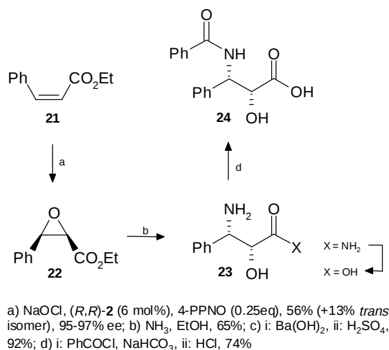
Scheme 6 Synthesis of the taxol side chain based on the enantioselective epoxidation of cis -cinnamate ethyl ester 21 .
