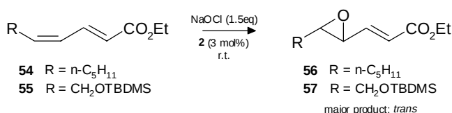
Scheme 10 Epoxidation of \alpha,\beta\text{-}\gamma,\delta -unsaturated esters.
